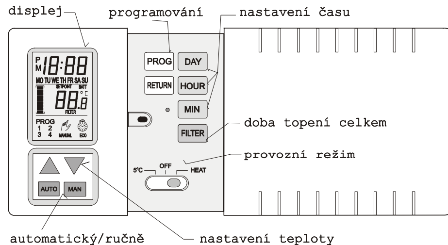
Obr. 1 Panel termostatu
