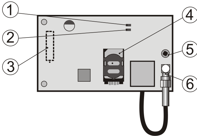
Fig. 1: JA-190Y communicator
