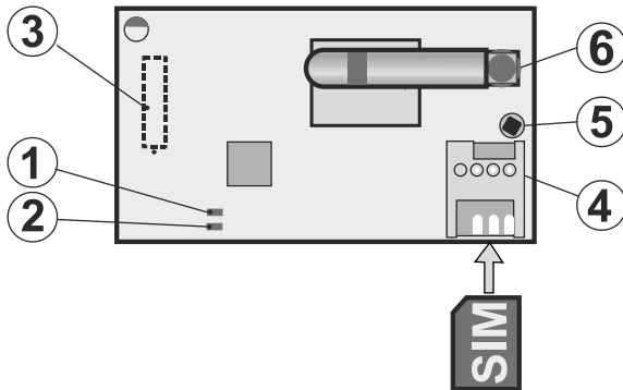
Fig. 1: JA-191Y Communicator
