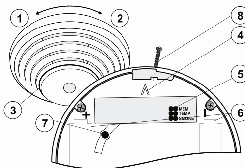
Fig. 6: 1 – detector cover opening; 2 – detector cover closing; 3 – optical status signalling (red LED); 4 – arrow showing where to insert the detector; 5 – configuration terminals; 6 – battery holders; 7 – button for test; 8 – locking screw;
